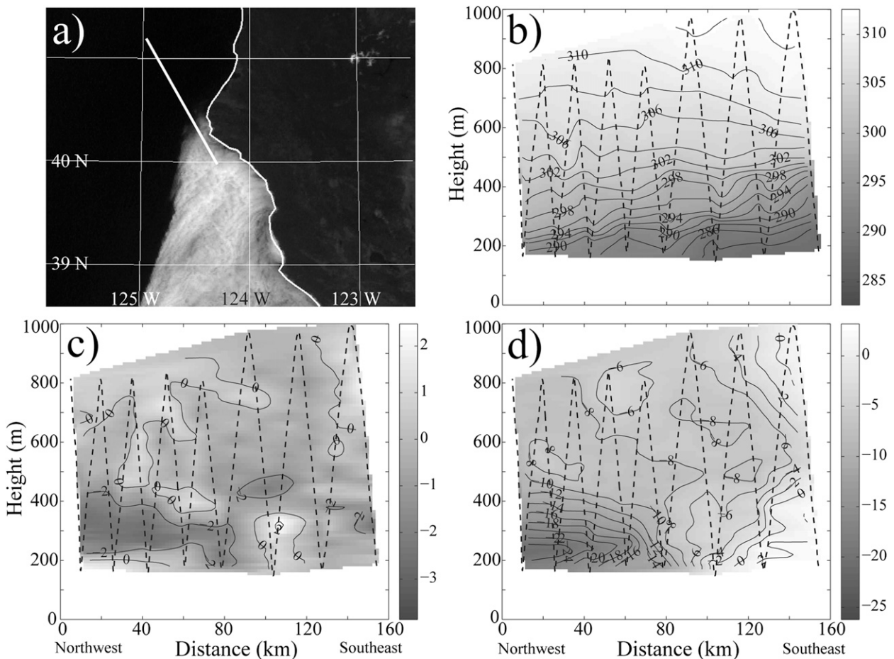
FIG. 9. As in Fig. 3, but for 1937–2015 UTC 25 Jun 2006.
